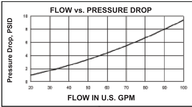
Figure 13_1 1/2" - Flow vs. Pressure Drop
