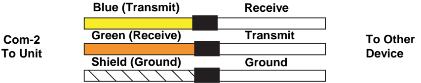
Com-2 wiring to exchange information with another device.
