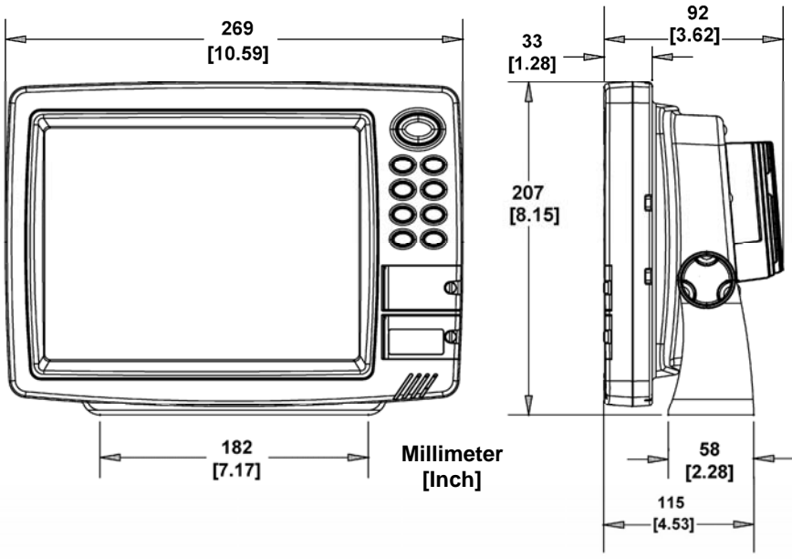
Front view (left) and side view (right) showing dimensions of the GlobalMap Baja 840c and mounted on gimbal brackets.
