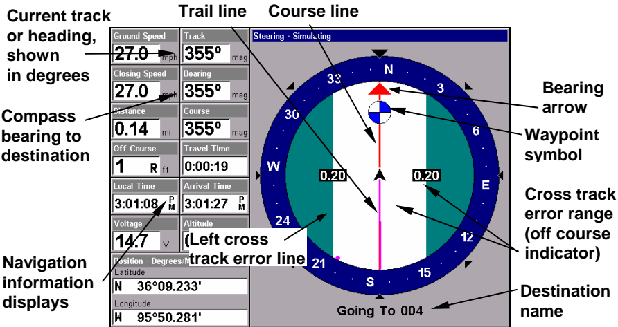
The GlobalMap Baja navigation page, backtracking a trail while creating a new trail.
