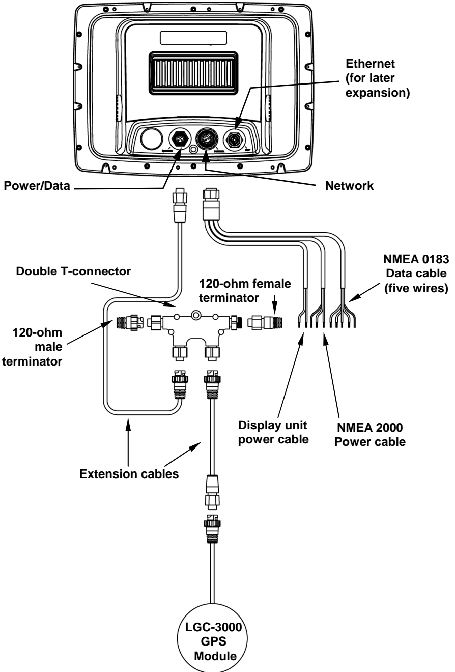
Cable connections, GlobalMap Baja 840c.
