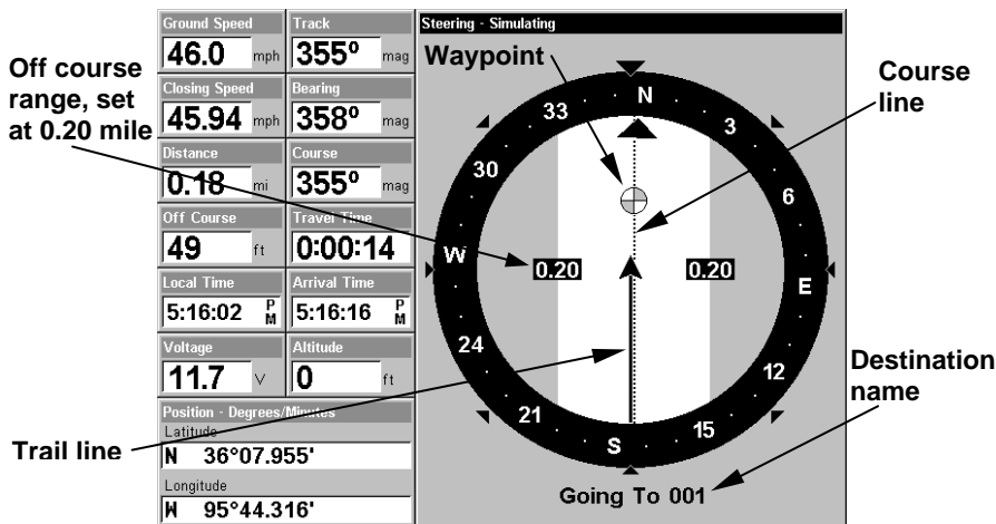
Navigation Page, navigating toward waypoint 001.
