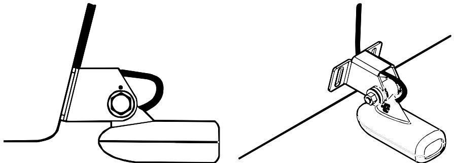
For single-frequency Skimmer, route cable over bolt and through bracket. Side view shown (left) and seen from above (right).
