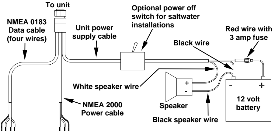
Connections for optional external speaker.
