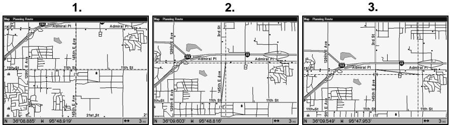
Route creation sequence, from left: (Fig. 1) Set route waypoint (1) at 11th St. & 145th Ave. (Fig. 2) Move cursor north to set point (2) at 145th & Admiral. (Fig. 3) With point (2) set, move cursor east to mark interstate on-ramp with waypoint (3). In figures 2 and 3, notice the rubber band line extending from the previously set waypoint to the cursor. This line will become the course for the route.
