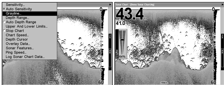
Grayline selected on sonar menu (left); Grayline control bar (right).
