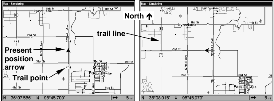
Navigate trail, map views: the driver (left) is northbound heading straight toward trail point 6. The northbound driver (right) has reached point 6 and has turned west to follow trail to point 7.
