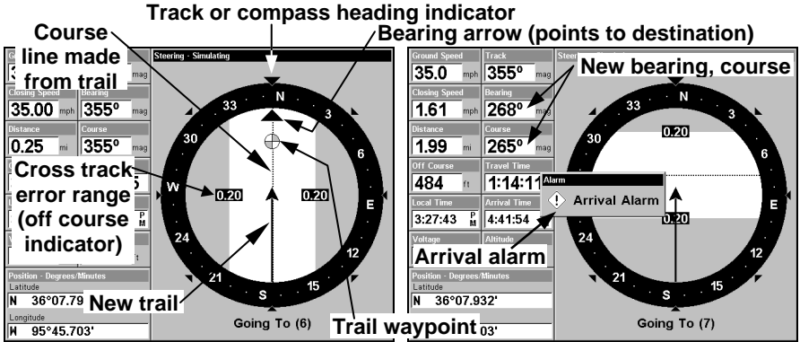
Navigate trail, map views: the driver (left) is northbound heading straight toward trail point 6. The northbound driver (right) has reached point 6 and has turned west to follow trail to point 7.
