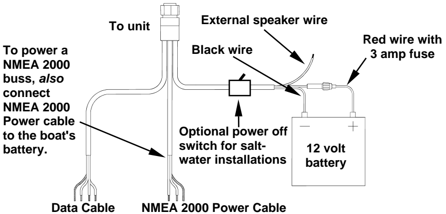
Power connections for LCX-17M sonar/GPS unit.
