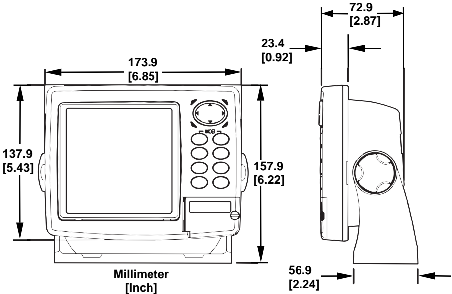
Front view (left) and side view (right) showing dimensions of the unit when mounted on gimbal bracket.
