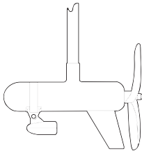
Transducer mounted on trolling motor, side view.
