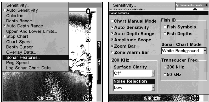
Sonar Menu with Sonar Features selected (left). In the Sonar Features menu, Noise Rejection (ASP) set to low setting (right).
