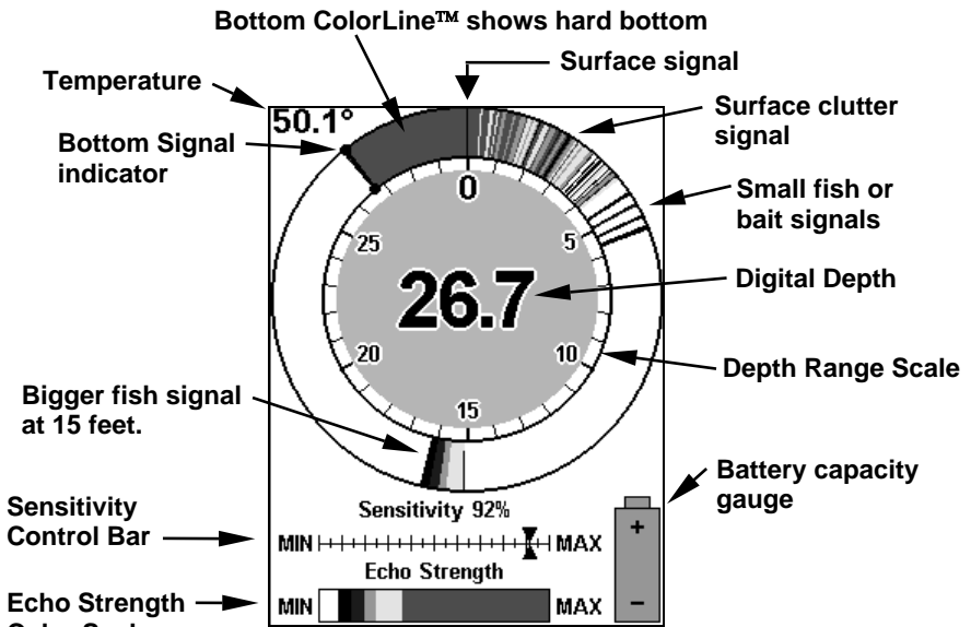
Ice Flasher page. Temp display requires optional TS-2U temp sensor.
