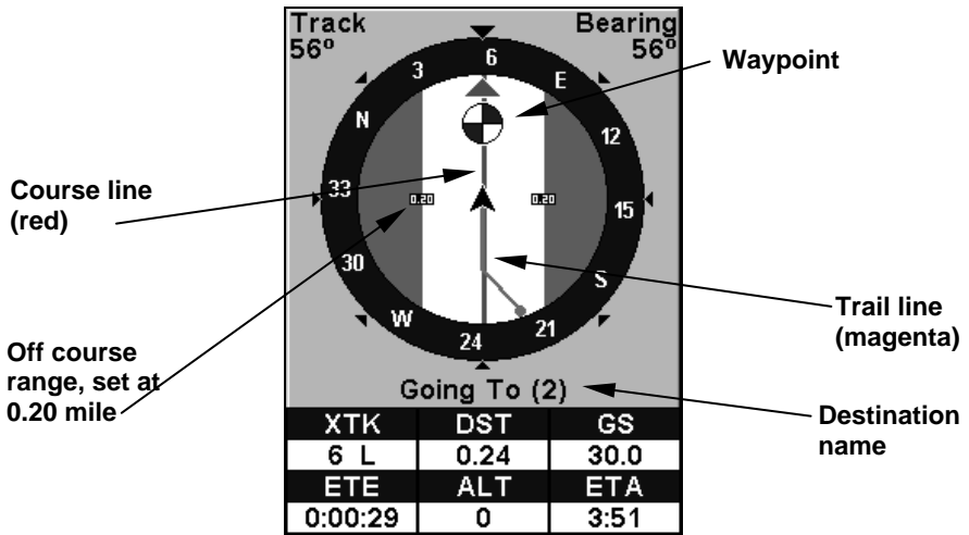
Navigation Page, navigating toward waypoint 2 and leaving a trail.
