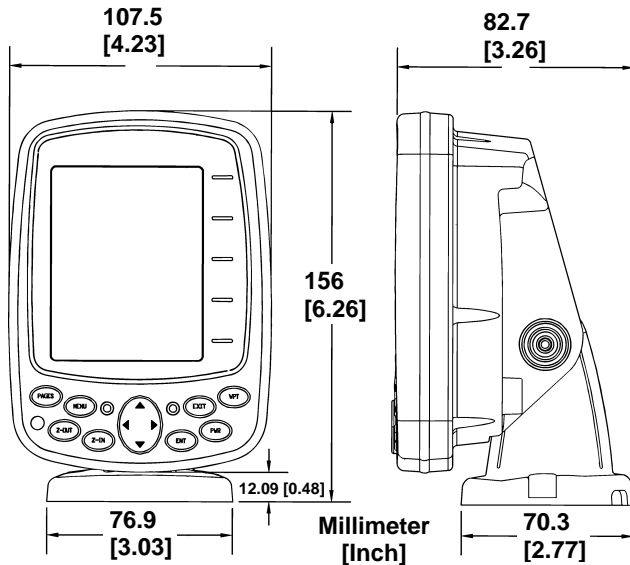
Front view (left) and side view (right) showing dimensions of the M68 when mounted on quick release bracket.
