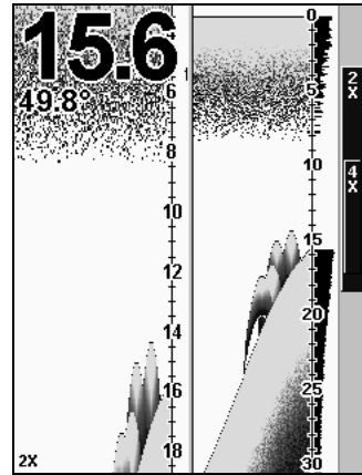
Sonar chart display options (from left) full sonar chart and split zoom.
