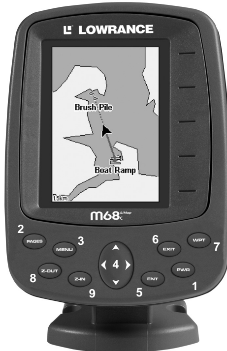
Lowrance M68 Sonar, front view, showing screen and keyboard. (A close-up of the keyboard can be found at the beginning of Sec. 7)
