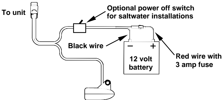
Power and transducer connections for the M68 sonar units (direct battery connection shown).
