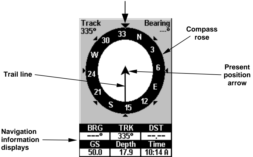
Navigation Page, recording a trail, traveling northwest. Page looks like this when the unit is not navigating to a waypoint, following a route, or backtracking a trail.
