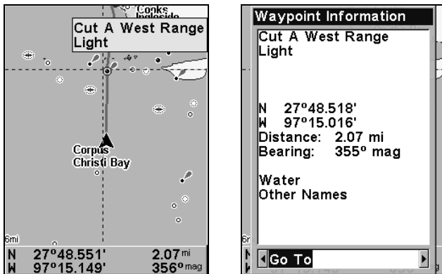
A Map Place selected by the cursor, left, Waypoint Information screen, right.
