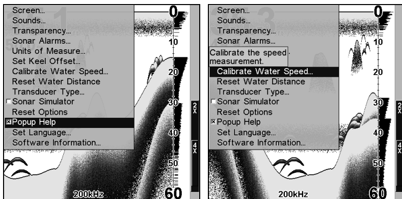
Main Menu, left, with Pop-up Help command highlighted. Right, this example shows the Pop-up Help message for the Calibrate Water Speed command, located on the Main Menu.
