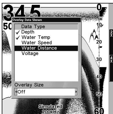
Data list showing "Water Speed" selected to display on Sonar Page.
