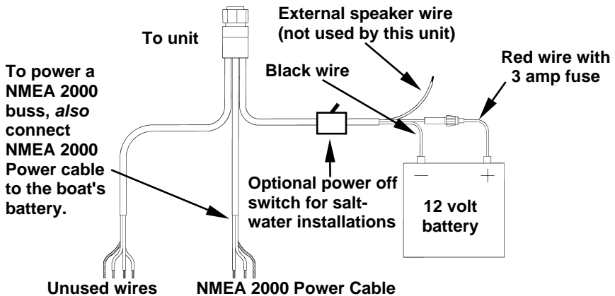
Power connections for X102C and X107CDF sonar units.
