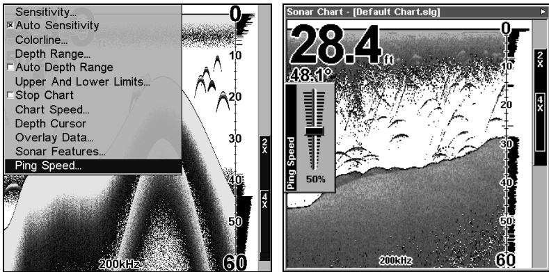
Left, Sonar Menu with Ping Speed command selected. Ping Speed Control Bar, right, at default setting.
