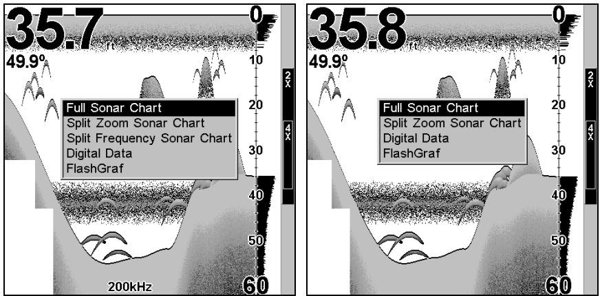
Pages Menu showing some Sonar display options (left, dual-frequency menu; right, single-frequency menu).
