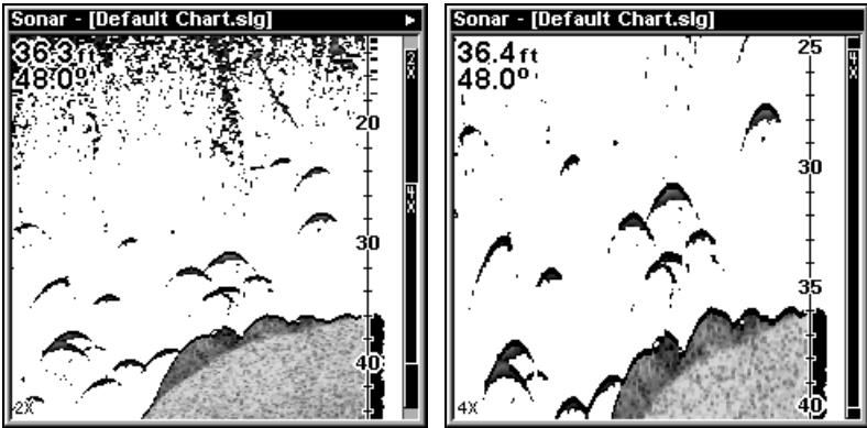
Left, full sonar chart zoomed 2X. Right, same view zoomed 4X.
