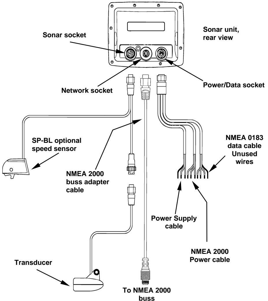
Sonar unit cable connections.
