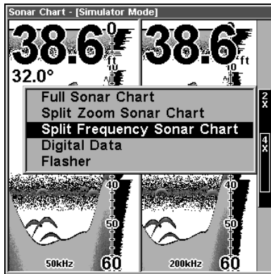
Split Frequency Sonar Chart page, with 50 kHz view (left) and 200 kHz view (right).
