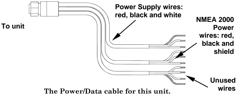
The Power/Data cable for this unit.
