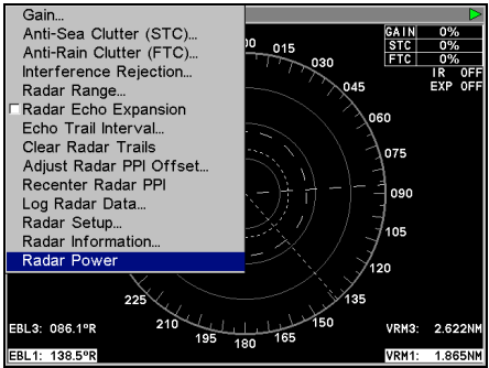
Radar only highlighted on Radar Pages menu (left). Radar menu with Radar Power selected (right).
