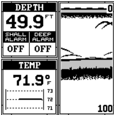
Window Group C
