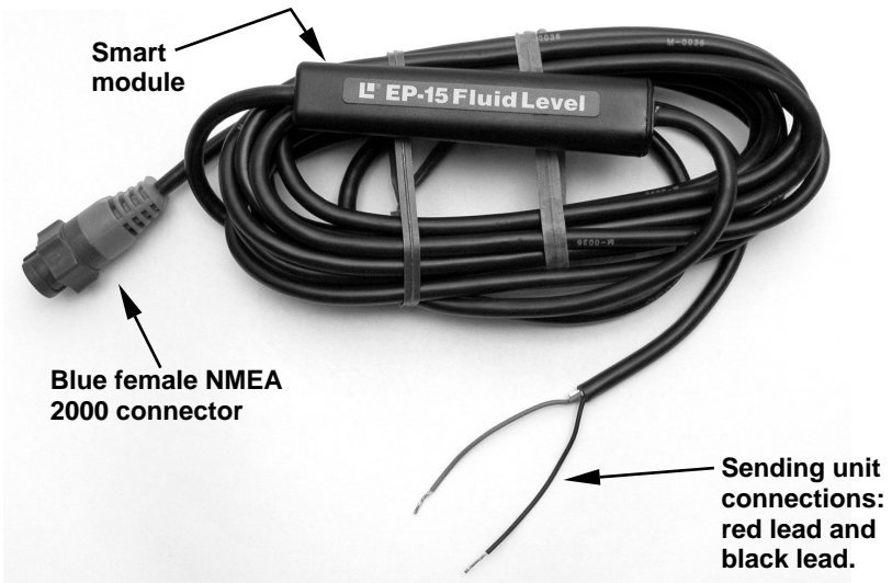
The EP-15 Fluid Level sensor.
