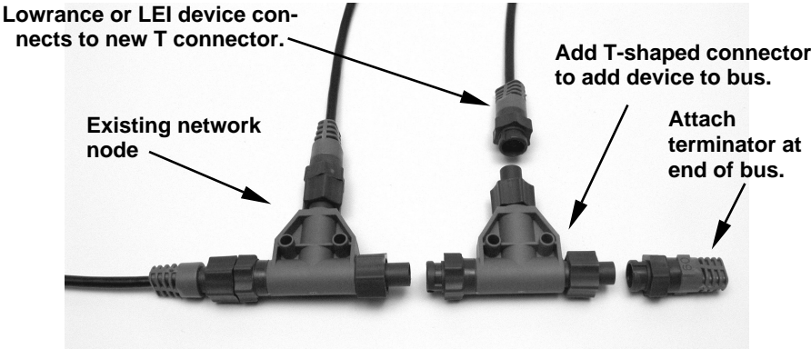
Add a new device to a NMEA 2000 bus by attaching a T connector between two T connectors, between a T connector and the end terminator, or between two backbone extension cables.
