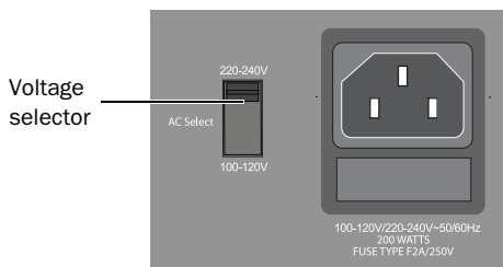
Voltage selector
