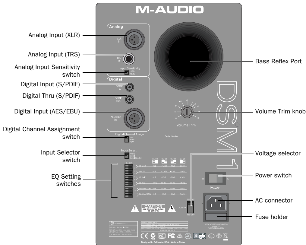
Figure 1. Back panel of the DSM1
