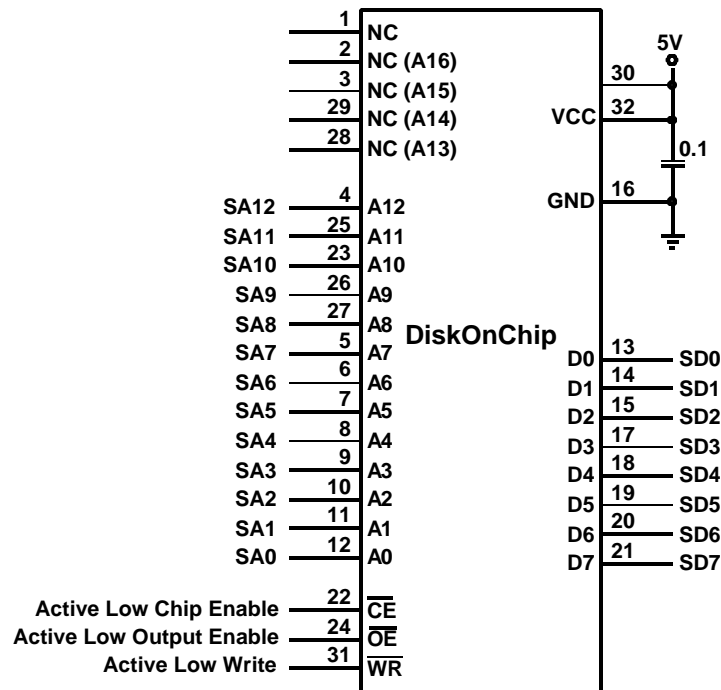
Figure 1: DiskOnChip Pins
