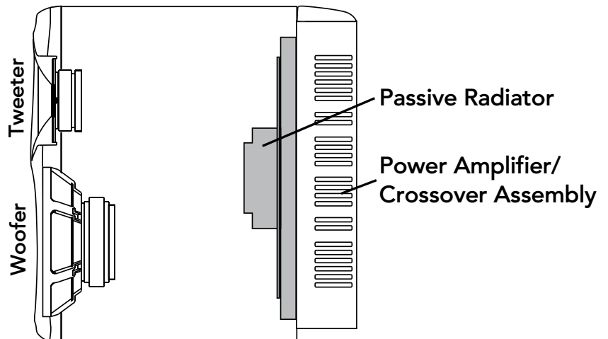
Figure 1. HR824 MK2 Cutaway side view
