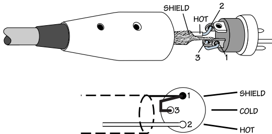
Unbalanced Male XLR Connector
