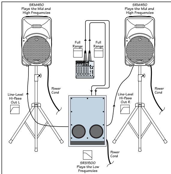
1 SRS1500 WITH 2 SRM450s
