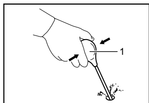
1. Blow-out bulb
