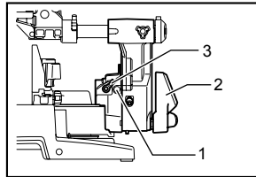
1. 0^\circ Angle adjusting bolt 2. Lever 3. Latch lever
