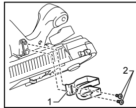
1. Hook 2. Screws
