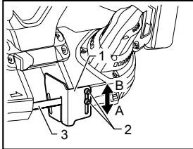
1. Stopper plate 2. Screws 3. Blade
