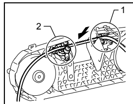
1. Lower holder 2. Upper holder
