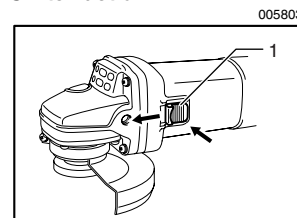
1. Switch lever
