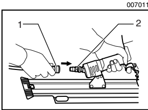
1. Air socket 2. Air fitting
