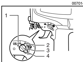
1. Continuous nailing 2. Trigger lock 3. Lock lever 4. Intermittent nailing
