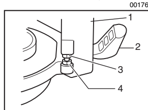
1. Arm 2. Lever 3. 0° adjusting bolt 4. Hex nut
