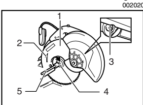
1. Blade case 2. Arrow 3. Shaft lock 4. Hex bolt 5. Socket wrench
