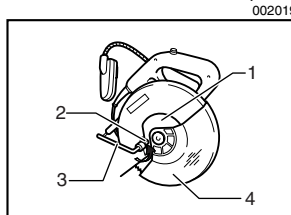
1. Center cover 2. Hex bolt 3. Socket wrench 4. Blade guard
