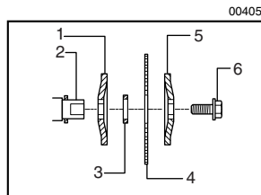
1. Inner flange 2. Spindle 3. Ring 4. Saw blade 5. Outer flange 6. Hex bolt (left-handed)
