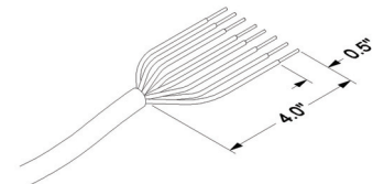
Figure 1 - CAT5 wire
