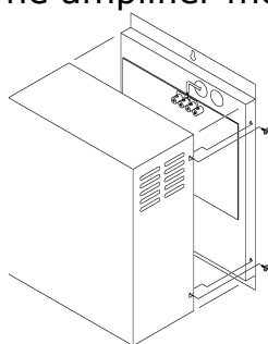
Figure 17 – Amplifier mounting
