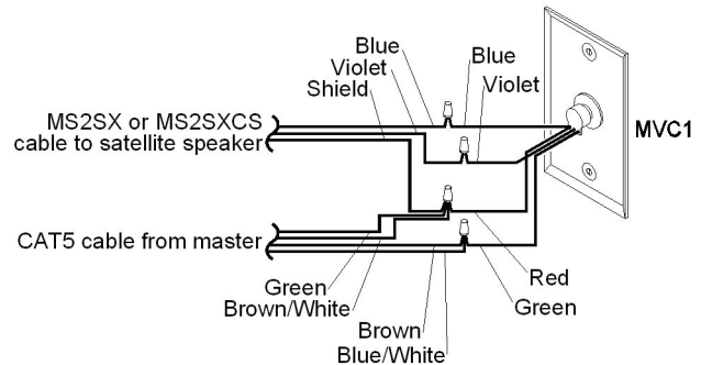
Figure 4 - Volume control wiring
