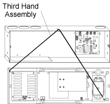
Figure 9 - Third hand assembly
