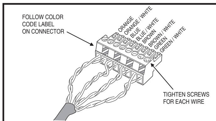
Figure 9. Completed Screw-down Connector Assembly
