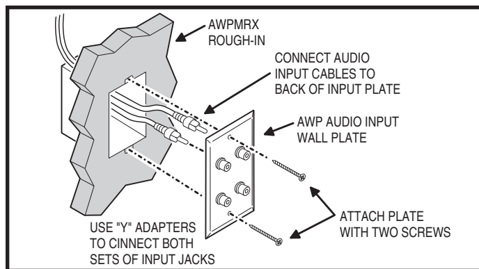
Figure 7. AWP Audio Wall Plate Wiring
