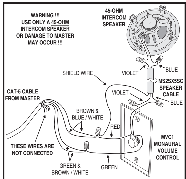
Figure 6. MVC-1 Volume Control Wiring
