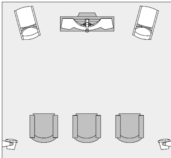
Figure 15. Ascent speakers as front channels, MartinLogan Theater as the center channel, MartinLogan Scripts as side surround (effects) channels.
