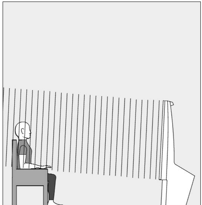
Figure 8. Your Ascent speaker system is a 48" inch line source when viewed vertically. Actual height above floor is from 16" inches to 64" inches.
