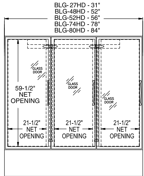
ELEVATION VIEW
