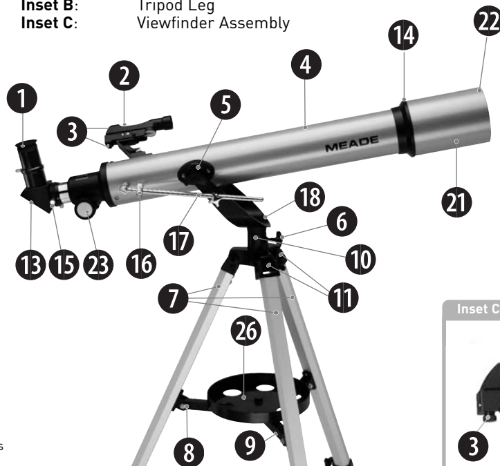
Figure 1: Meade 70AZ-AR Altazimuth Refracting Telescope
