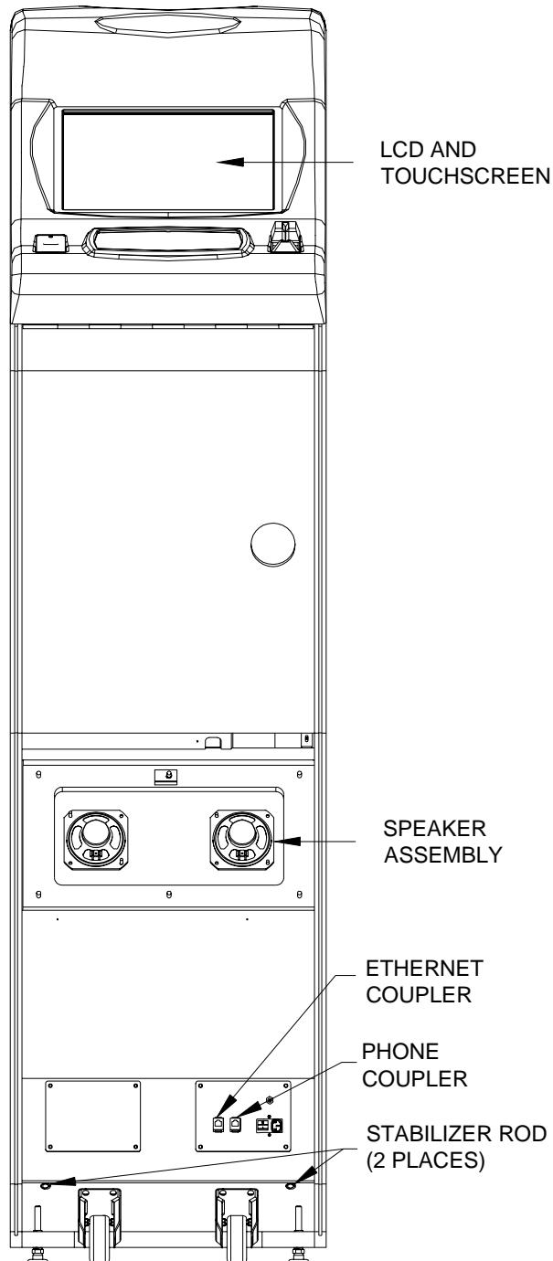
FIGURE 25 - REAR VIEW OF THE FUSION WITH BEZEL OPEN
