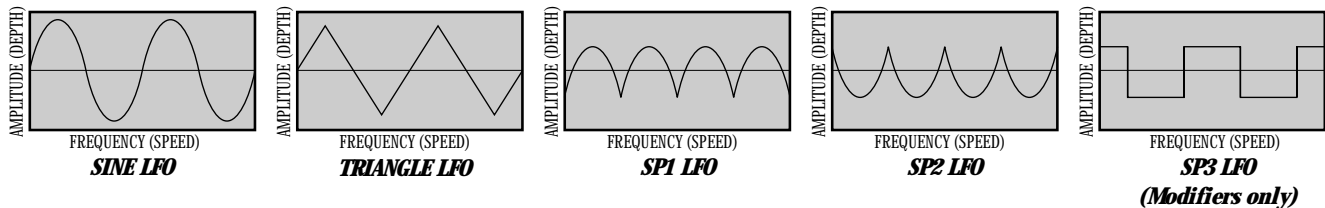
Figure 4-2 LFO Types
