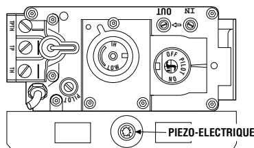
VANNE GAZ MILLIVOLT SIT
