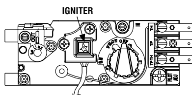
HONEYWELL MILLIVOLT GAS VALVE
