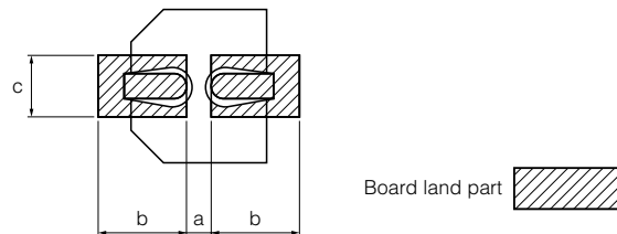
[ Table of Board Land Size vs. Capacitor Size ]
