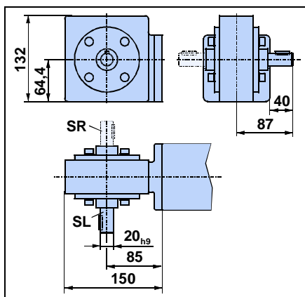
SL: shaft on left SR: shaft on right
