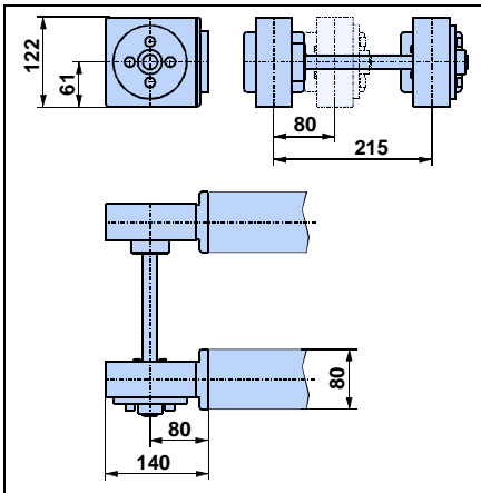
Centre distance A between 80-215 mm
