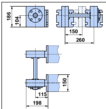
Centre distance A between 150-260 mm
