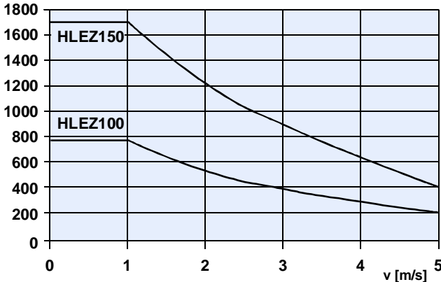
F_z [N]
