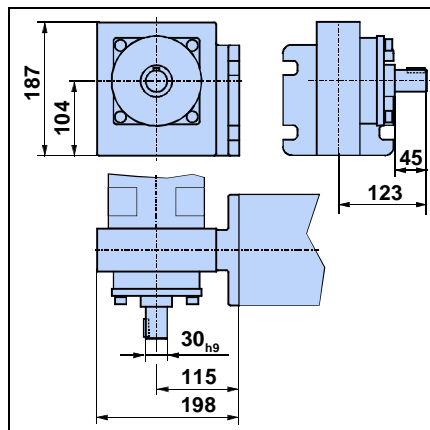
RL: gearbox on right and shaft on left LR: gearbox on left and shaft on right
