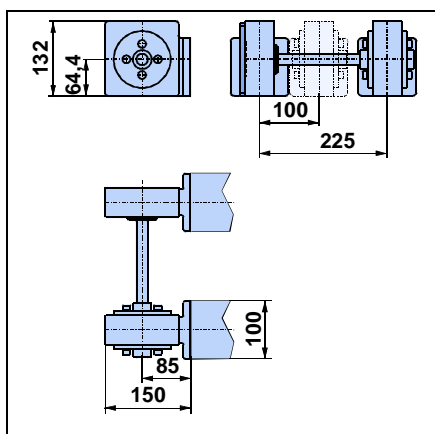
Centre distance A between 100-225 mm
