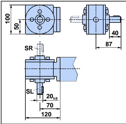
SL: shaft on left SR: shaft on right
