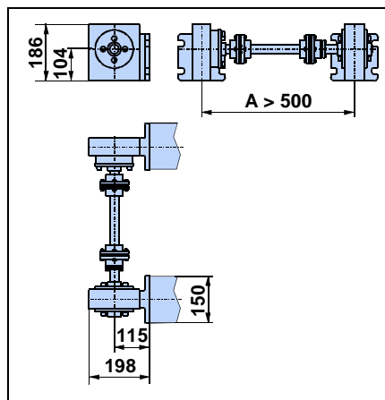
Centre distance A greater than 500 mm
