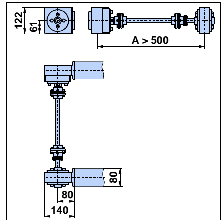
Centre distance A greater than 500 mm
