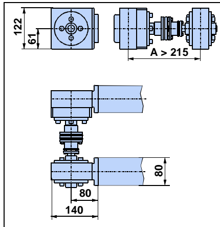
Centre distance A between 215-500 mm
