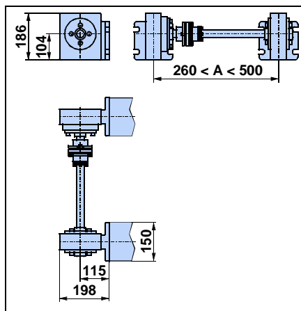
Centre distance A between 260-500 mm
