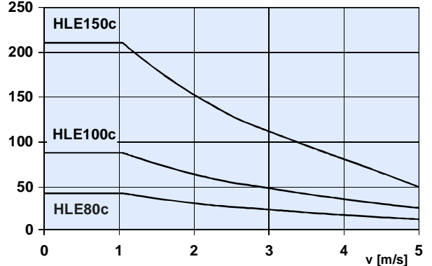
M_z [Nm]
