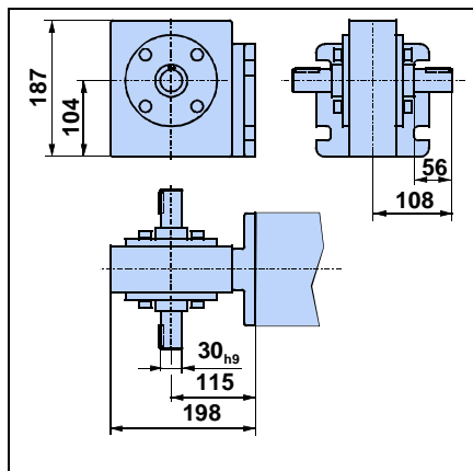
SB: shaft on both sides
