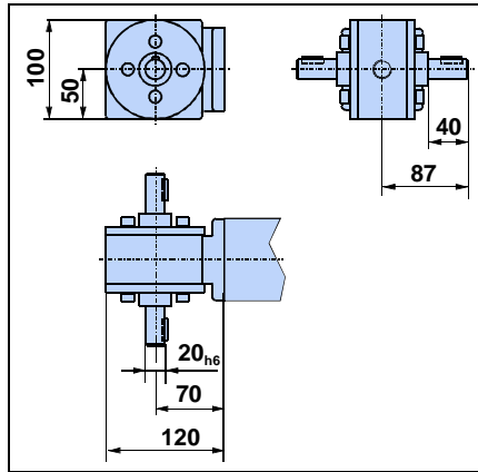
SB: shafts on both sides
