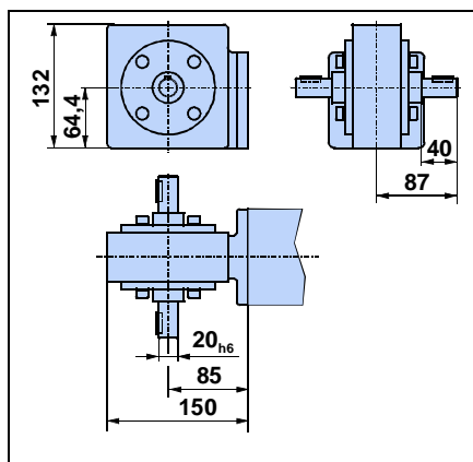
SB: shaft on both sides
