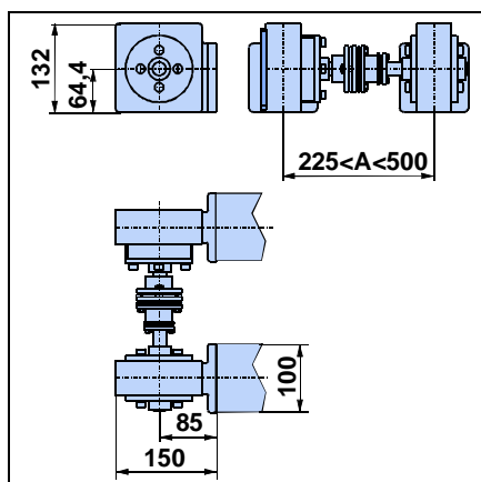
Centre distance A between 225-500 mm
