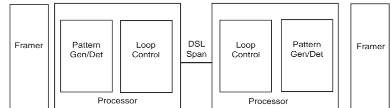
Figure 8: Block Diagram Two Model 1089s Communicating over the DSL Span
