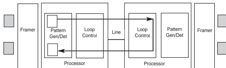
Figure 9: Block Diagram Two Model 1089s Communicating over the DSL Span
