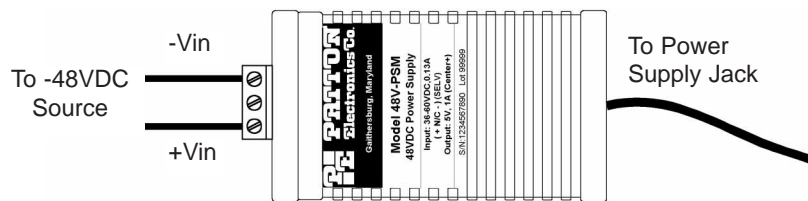
Figure 6. Connecting DC Power to the 48V-PSM DC Power Supply.
