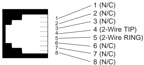
Figure 4. Model 1089 twisted pair line interface.
