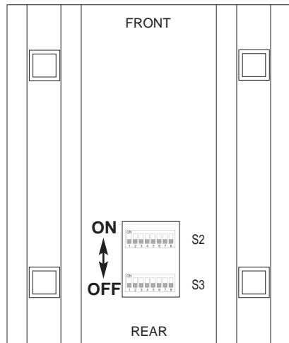
Figure 1. Underside of Model 1089 Series, showing location of DIP switches
