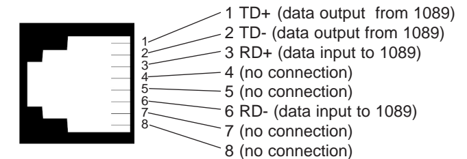
Figure 5. Model 1089 10BaseT Ethernet RJ-45 Connector Pinout
