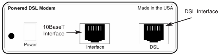
Figure 3. Model 1089 Rear Panel
