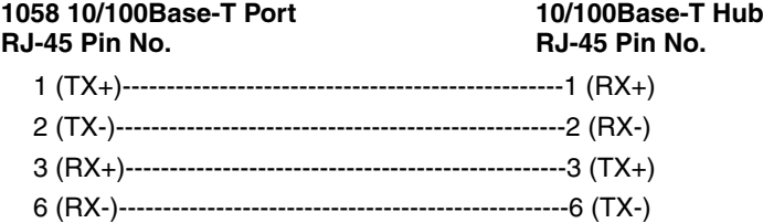
Figure 6. Wiring diagram for connecting the Model 1058 to a 10/100Base-T hub
