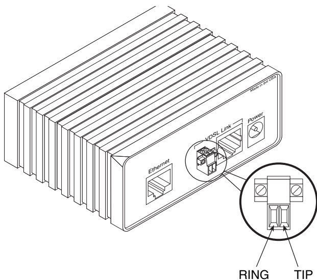
Figure 4. Model 1058D (Terminal Block) twisted pair line interface.
