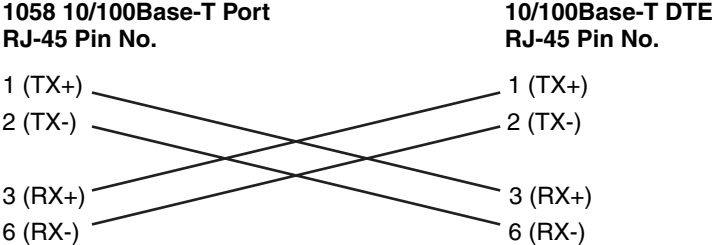
Figure 7. 10/100Base-T crossover cable
