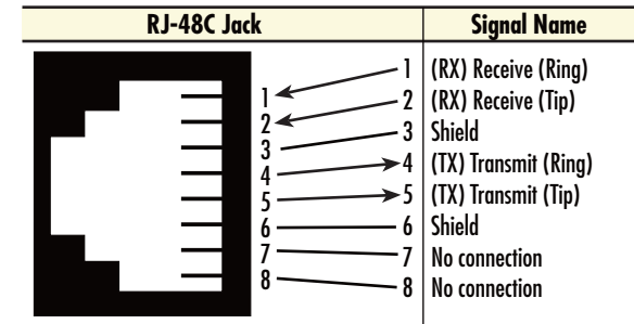
Figure 3. Model 2702 twisted pair line interface.
