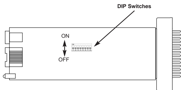
Figure 1. Model 2702 bottom view, showing location of DIP switches
