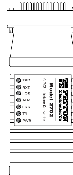
Figure 4. Top of Model 2702, Showing LED Indicators
