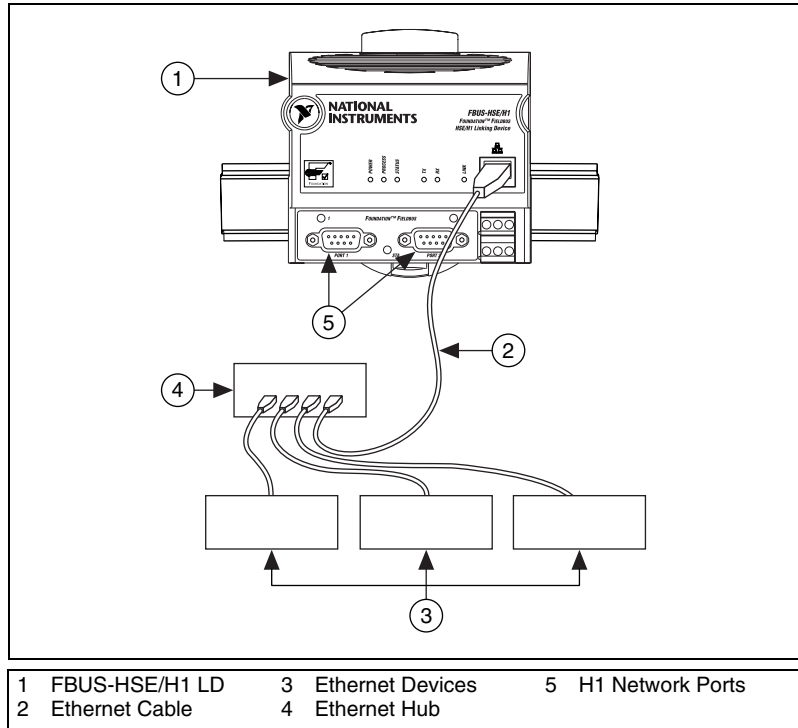
Figure 1-1. Typical Ethernet Network Setup
