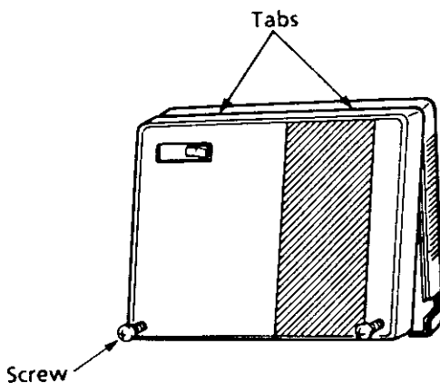
Figure 200-15 Replacing the KSU cover
