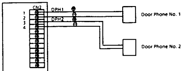
Figure 200-38 Door Phone Connection
