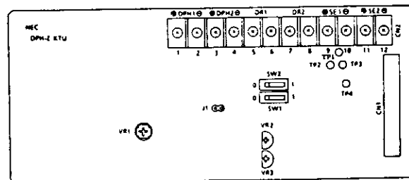
Figure 200-37 DPH-Z KTU Switch and Connector Layout
