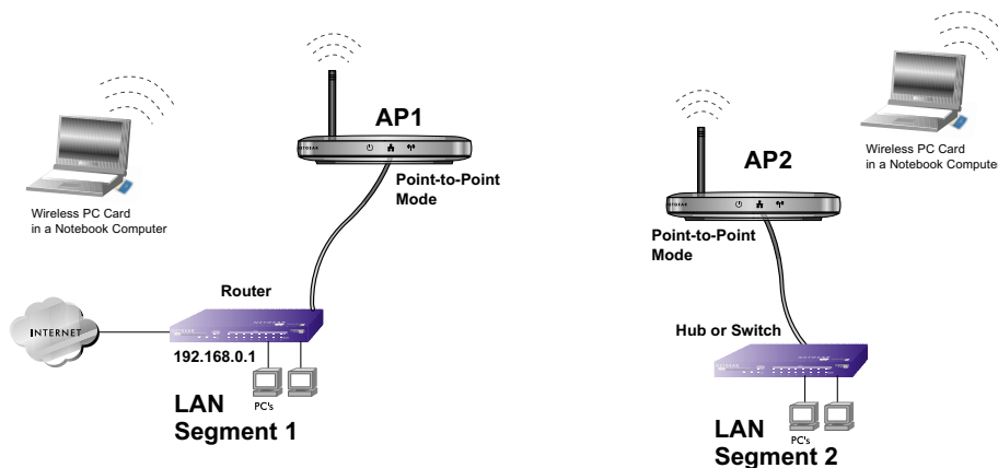
Figure 5-3: Wireless point-to-point bridging
