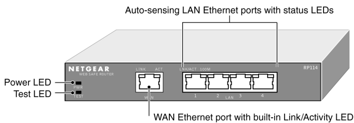
Figure 2-1. RP114 Front Panel
