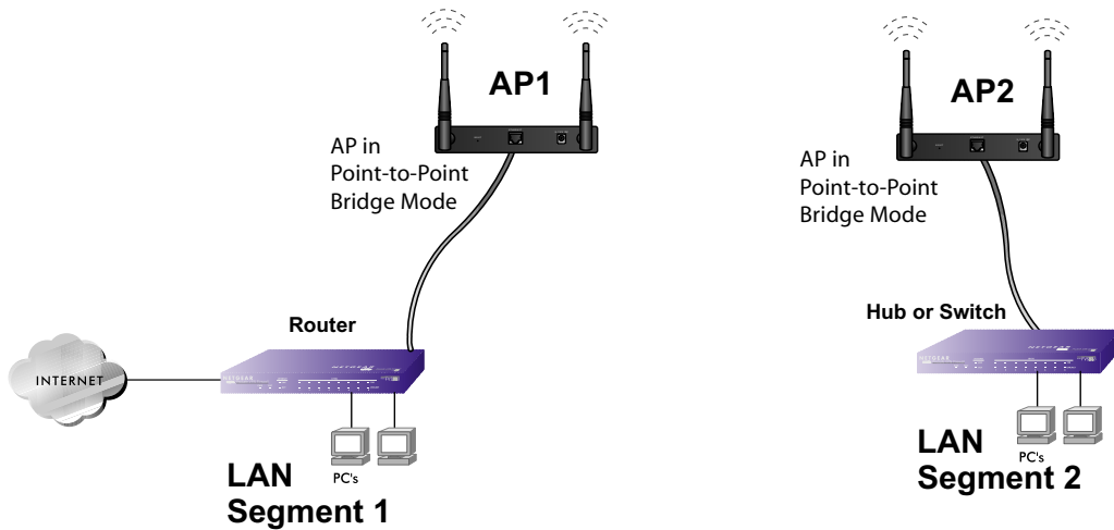
Figure 5-7: Point-to-Point Bridge
