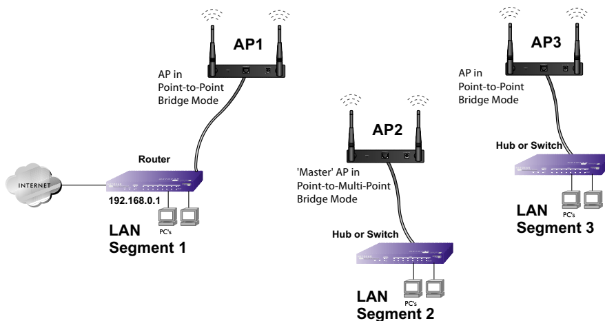
Figure 5-8: Multi-Point bridging
