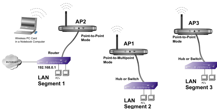
Figure 5-4: Wireless Bridging
