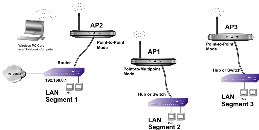
Figure 5-3: Wireless Bridging
