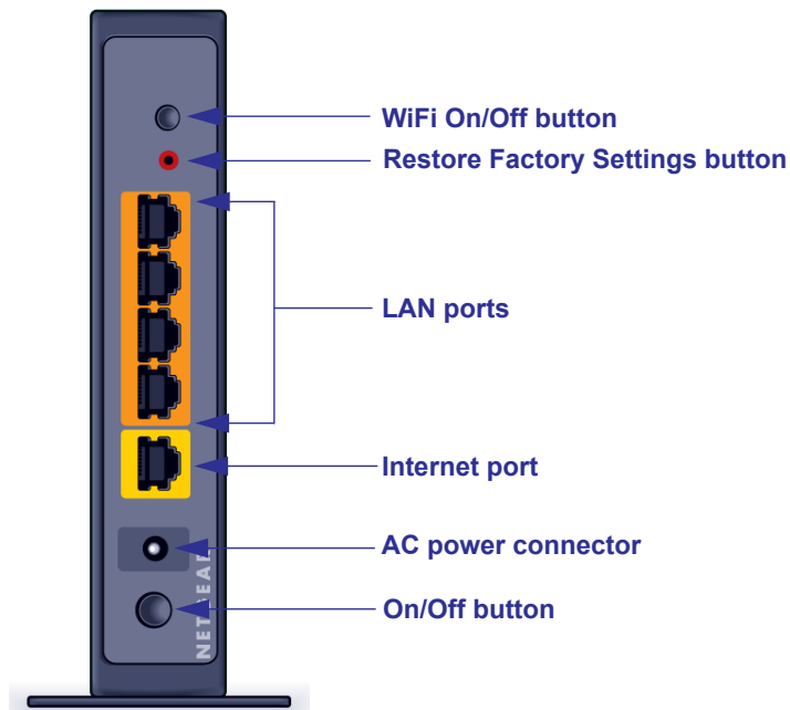
Figure 3. Back panel
