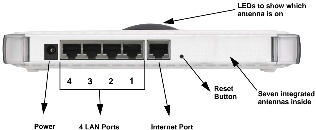
Figure 1-2: WPN824 Rear Panel
