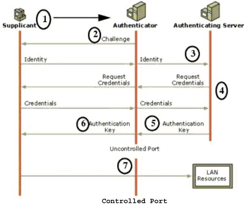
Figure D-4: 802.1x Authentication Sequence
