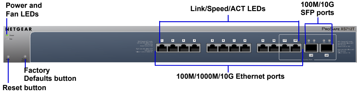
Figure 2. Front panel
