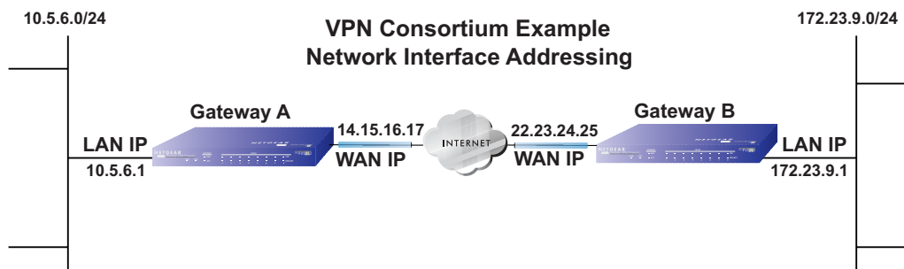
Figure C-4: VPN Consortium example network interface addressing
