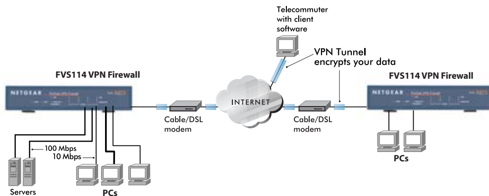
Figure 6-1: Secure access through FVS114 VPN firewalls
