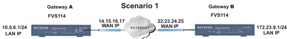
Figure 6-6: LAN to LAN VPN access from an FVS114 to an FVS114
