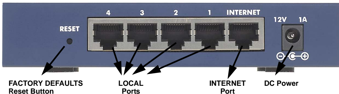
Figure 2-2: FVS114 rear panel
