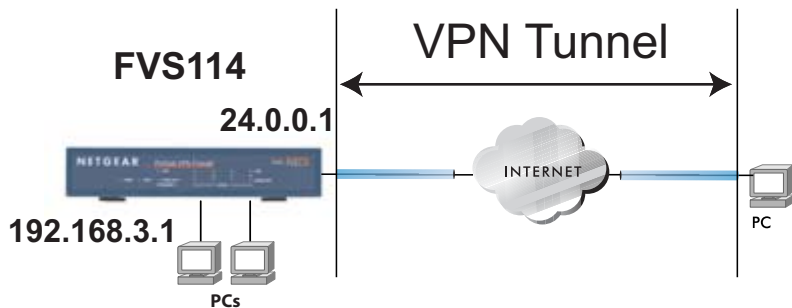
Figure 5-1: Client-to-gateway VPN tunnel
