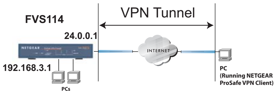
Figure 5-3: Client-to-gateway VPN tunnel
