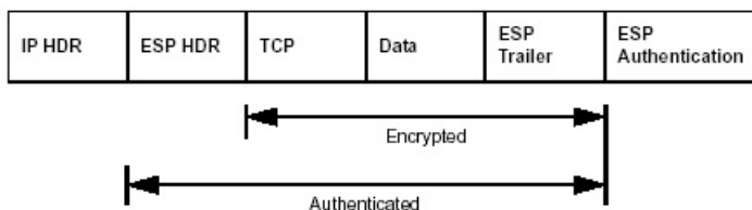
Figure C-1: Original packet and packet with IPSec Encapsulated Security Payload
