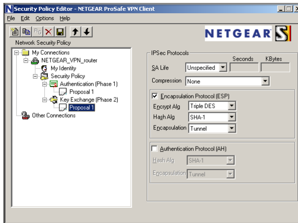
Figure 5-15: Security Policy Editor Key Exchange
