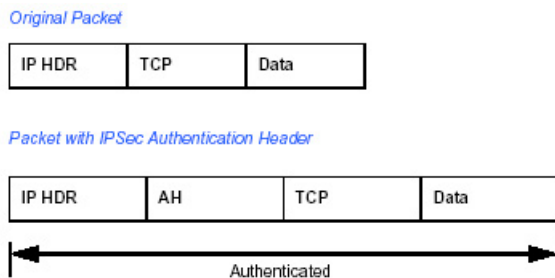
Figure C-2: Original packet and packet with IPSec Authentication Header
