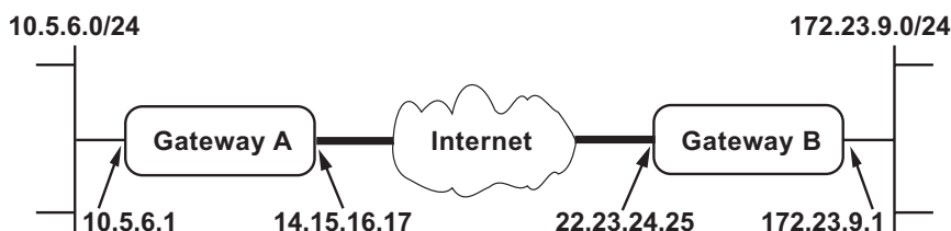
Figure 6-5: VPN Consortium Scenario 1
