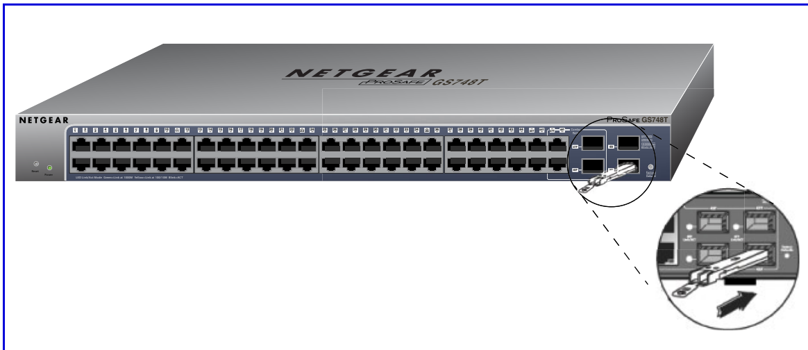
Figure 8. Install an SFP Transceiver Module
