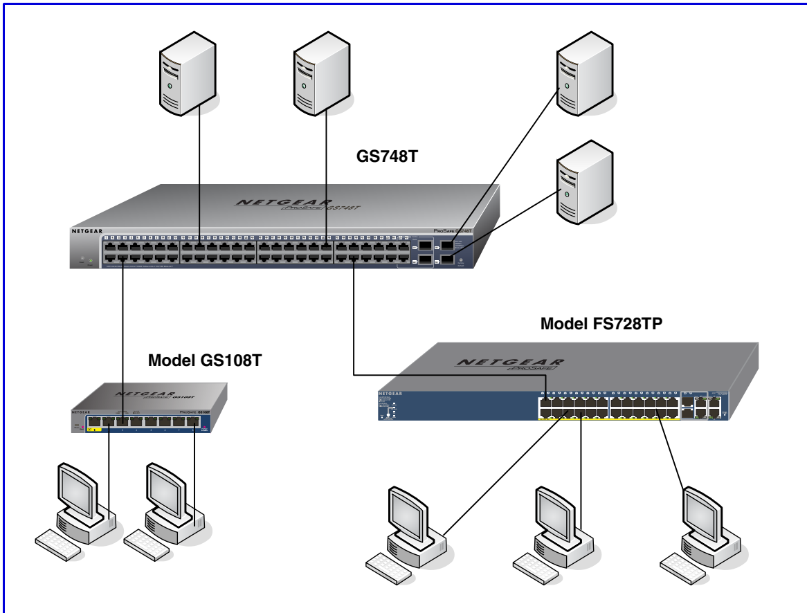
Figure 5. Backbone Switching
