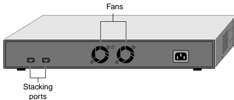
Figure 2-2. Front and Back Panels of the FS524S Switch
