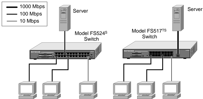
Figure 3-1. Example of Desktop Switching
