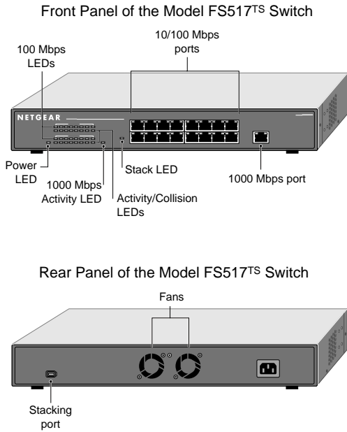
Figure 2-1. Front and Back Panels of the FS517TS Switch
