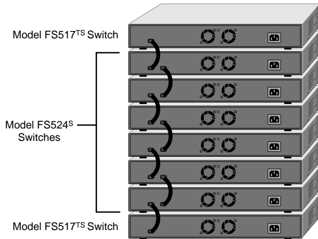
Figure 4-5. Cabling FS517TS and FS524S Switches
