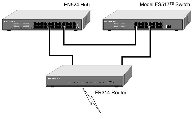
Figure 2-4. Warning! Creating loops disables your network (Example 2)
