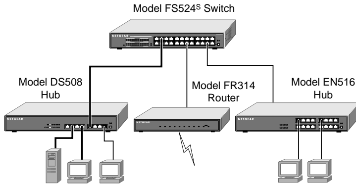
Figure 3-2. Example of Segment Switching and Bridging
