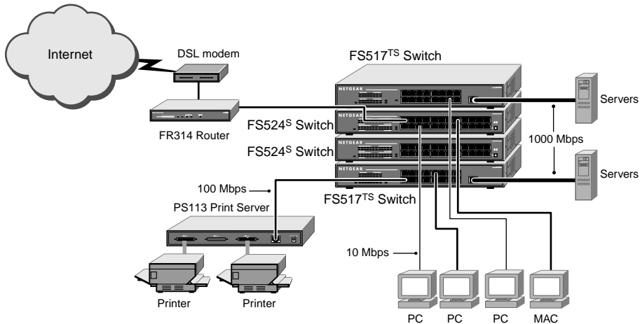
Figure 3-3. Example of Switched Stacking
