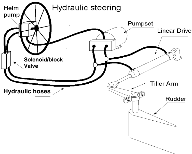
Figure 2: Typical installation on boat with hydraulic steering, including Pumpset PF-03.
