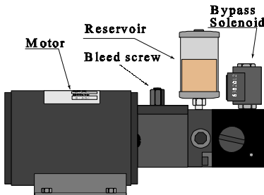
Pumpset PF-0,3S with solenoid and reservoir
