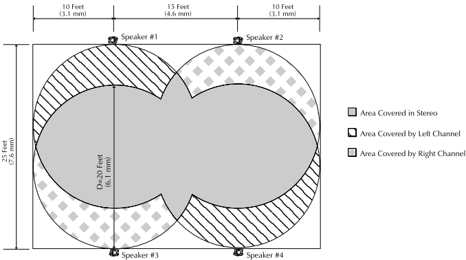
Figure 1 Stereo Coverage 4 speakers
