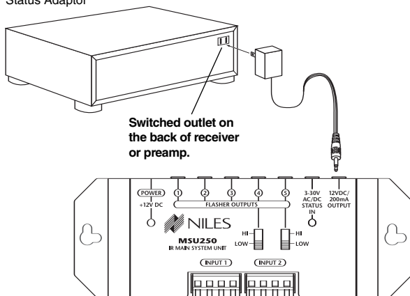
Figure 12: Connecting the Status Adaptor
