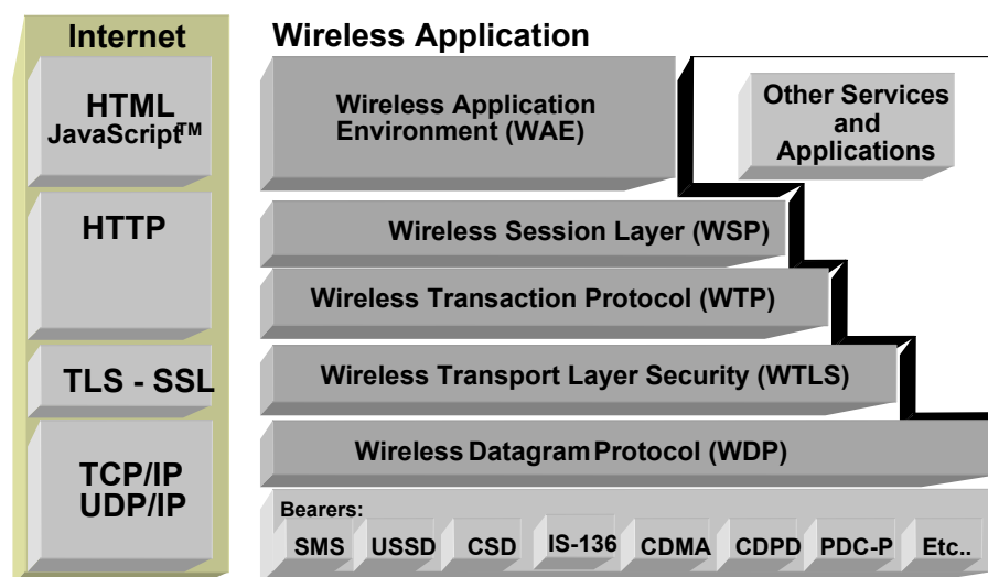
Figure 1A: Comparison of Internet and WAP architecture
